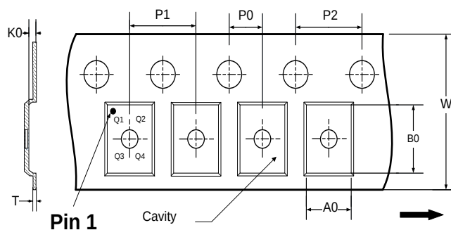
TAPE DIMENSIONS
